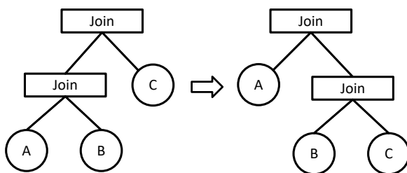
Figure 4.5: Join right associativity
