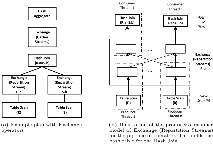
Figure 2.9: Parallelism using Exchange operators
