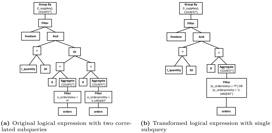
Figure 4.16: Transform a query with two EXISTS subqueries into a query with a single EXISTS subquery.
