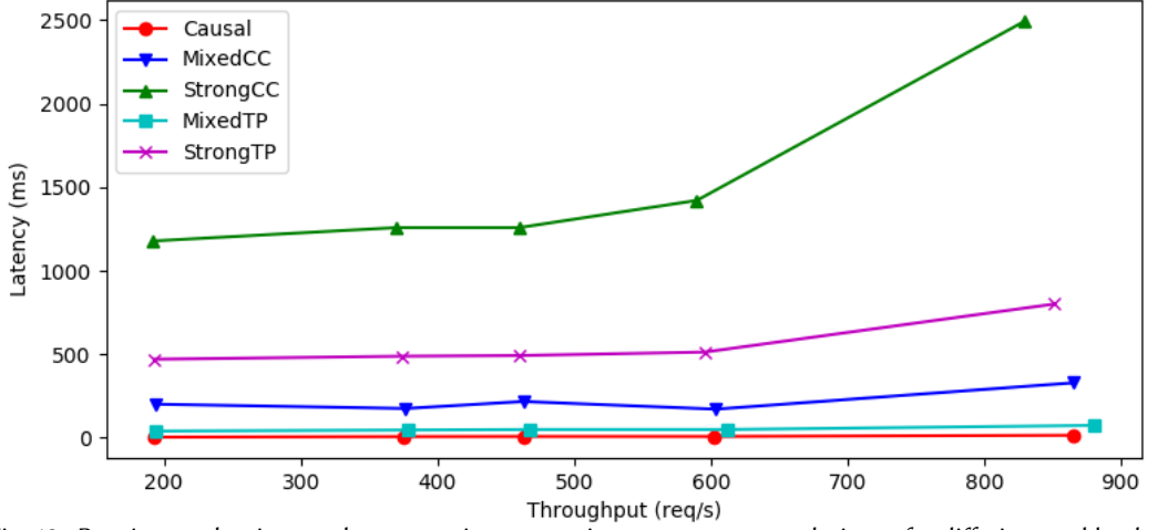
Fig. 12. Runtime evaluation results, comparing contention-management techniques for differing workloads. CC refers to the congestion control technique and TP to token passing. Causal refers to workloads including no guards, mixed to mixed-consistency workloads, and strong to workloads in which all operations conflict.
