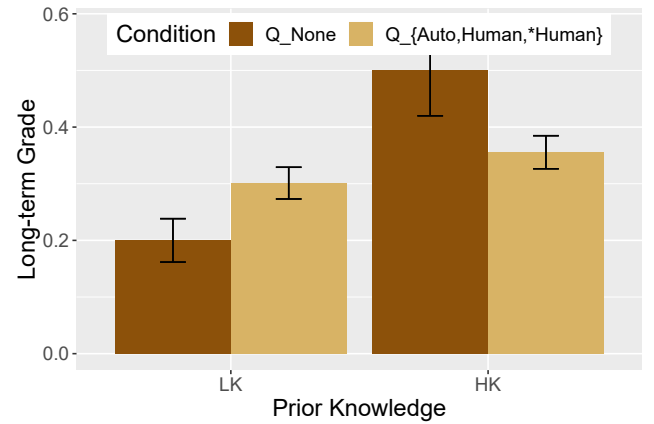
Figure 3: Long-term grades by non-question vs. question condition and prior knowledge level. LK participants particularly benefit in the case of interactive questions.
