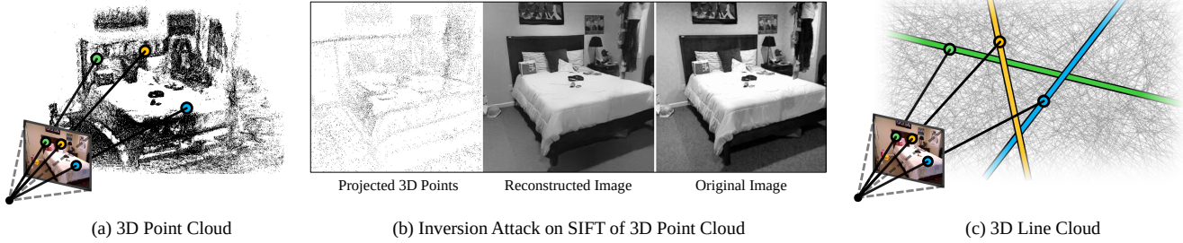
Figure 1: (a) Traditional image-based localization using 3D point cloud, which reveals potentially confidential information in the scene. (b) Reconstructed image using projected sparse 3D points and their SIFT features [50]. (c) Our proposed 3D line cloud protects user privacy by concealing the scene geometry and preventing inversion attacks, while still enabling accurate and efficient localization.
