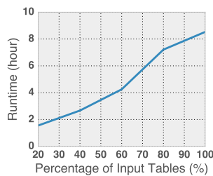
Figure 9: Scalability.
