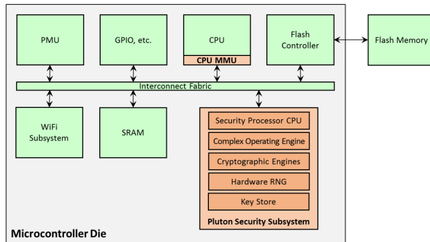
Figure 2. Architecture of the Experimental Sopris Highly Secure WiFi-enabled Microcontroller.
